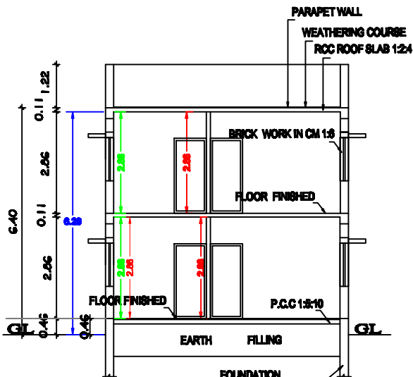
SECTION "A-B"
