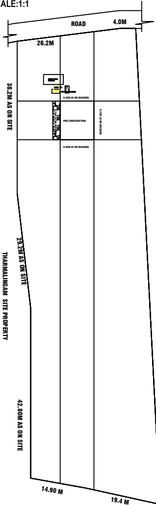
VENKIDUSAMY SITE PROPERTY
