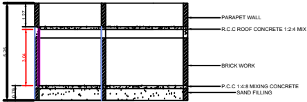
CROSS SECTION
