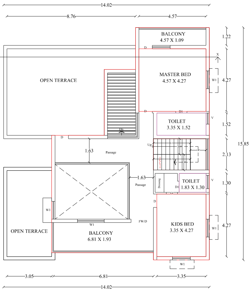
PRO.FIRST FOOR PLAN
