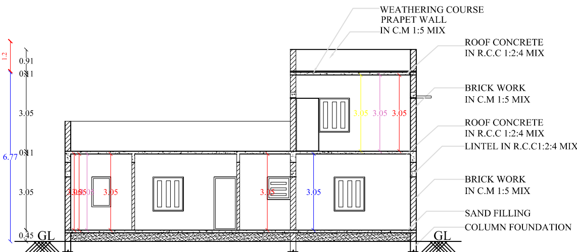
SECTION ON"XX"
