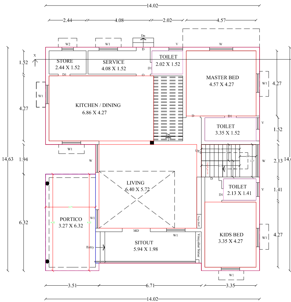
PRO.GROUND FOOR PLAN
