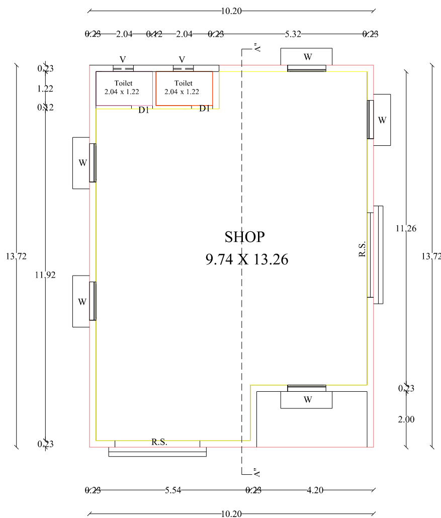
PRO.GROUND FLOOR
