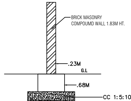
TAILS OF COMPOUND WALL
