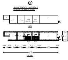
WASTE WATER RECYCLING SYSTEM:
