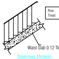
Staircase Details
