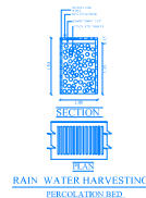
RAIN WATER HARVESTING CIRCULATION SYSTEM
