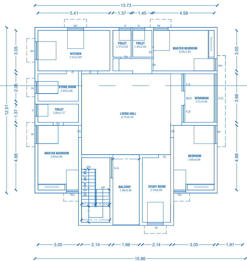
TYPICAL_FLOOR_PLAN=1,2
