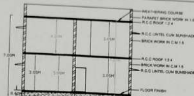
SECTION ON XX
