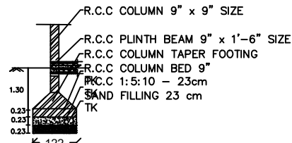
SECTION COLUMN DETAILS PLAN
