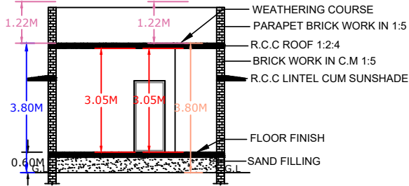
SECTION ON XX
