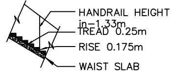
STAIRCASE DETAILS
