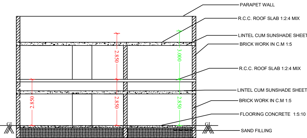
SECTION
