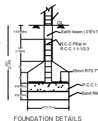
FOUNDATION DETAILS
