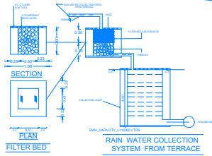
RAIN WATER COLLECTION SYSTEM FROM TERRACE
