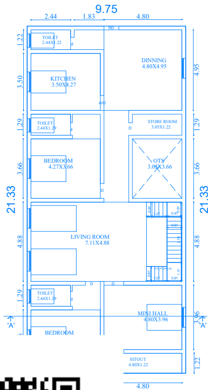
OR PLAN
