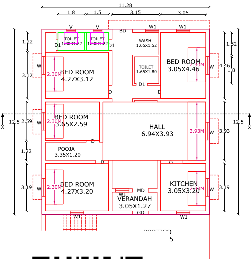
FLOOR PLAN
