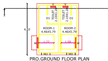
PRO.GROUND FLOOR PLAN BLOCK-2
