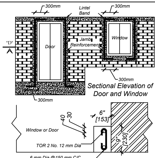
Typical Details of Providing Vertical Steel Bars Around Door / Windows
