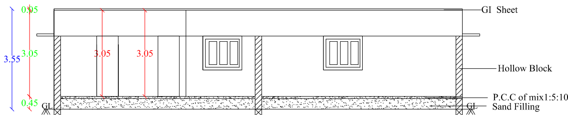
SECTION-XX
