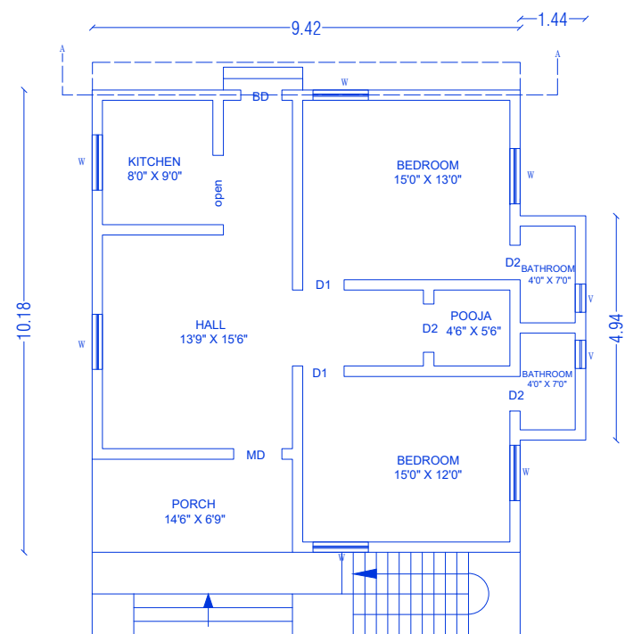
PRO-GROUND FLOOR
