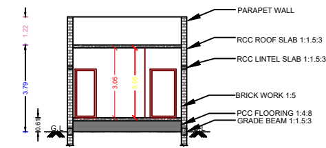
SECTION AT AB
