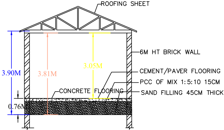
CROSS SECTION ON XX
