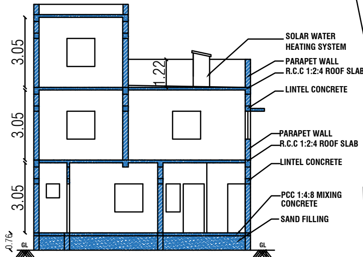
SECTION NO - "AB"
