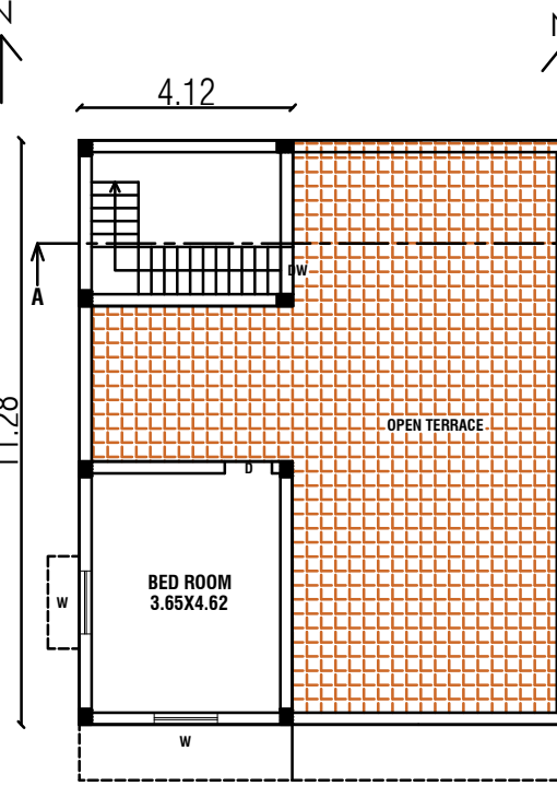
PRO.SECOND FLOOR PLAN
