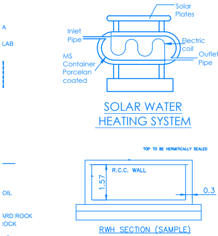
RWH_CAPACITY_L = 2000LTRS
