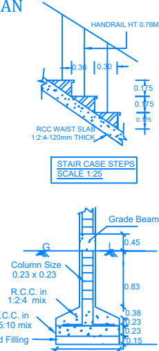
COLUMN DETAILS NOT TO SCALE
