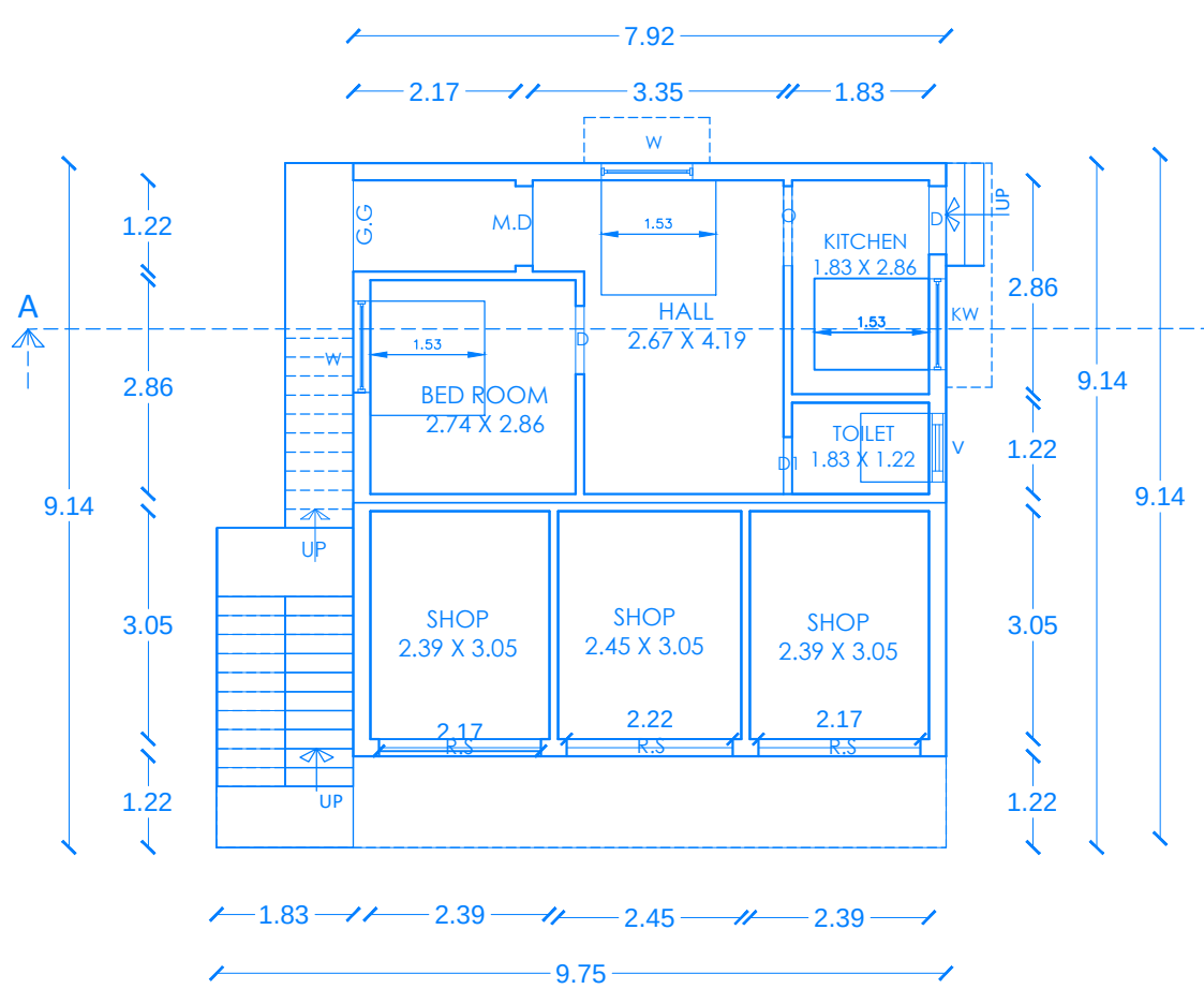
LOOR PLAN
