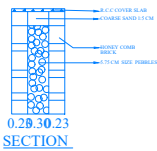
RAIN WATER HARVESTING I.PERCOLATION PIT
