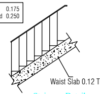
Staircase Details
