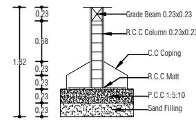
Foundation Detail
