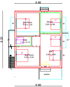
PRO. GROUND FLOOR PLAN
