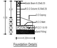
Foundation Details
