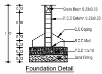
Foundation Detail
