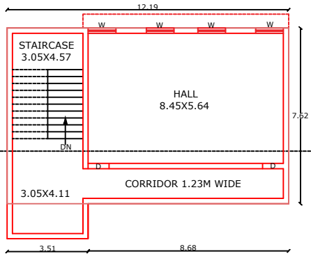
PRO.SECOND FLOOR PLAN
