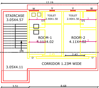
EXT.FIRST FLOOR PLAN
