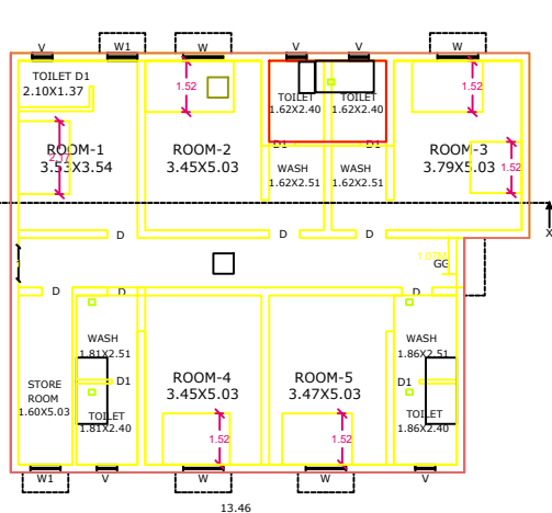
EXT.FIRST FLOOR PLAN
