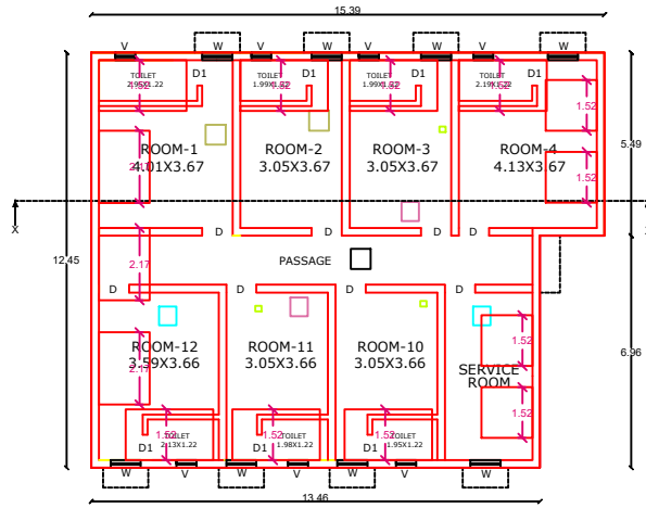
PRO.SECOND FLOOR PLAN
