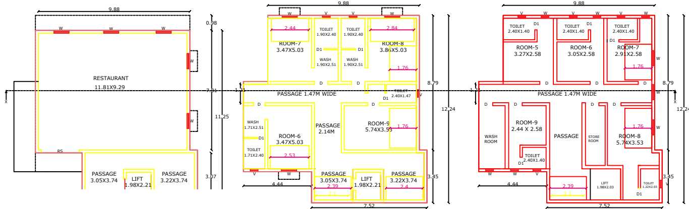
EXT.FIRST FLOOR PLAN
