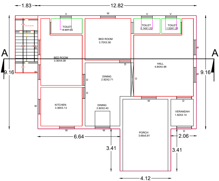
EX.GROUND FLOOR PLAN
