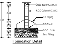
Foundation Detail
