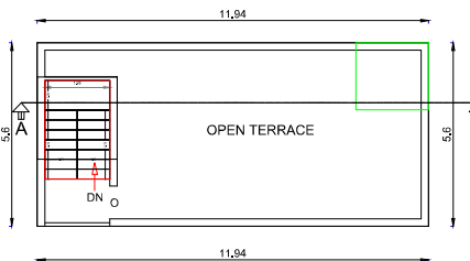
TERRACE FLOOR PLAN PROPOSED
