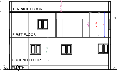
SECTION ON AB PROPOSED
