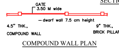
COMPOUND WALL PLAN
