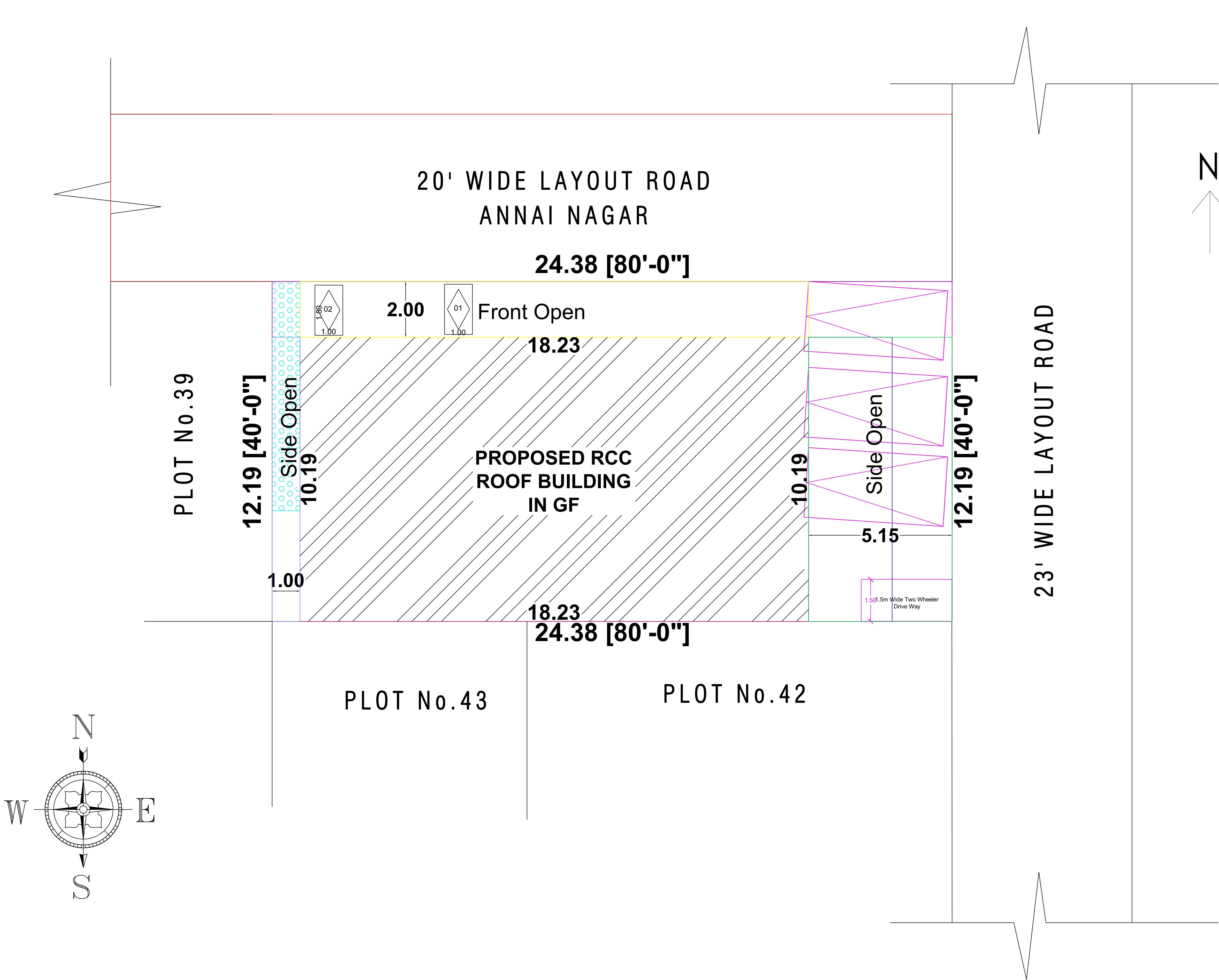
SITE PLAN [1:100]
