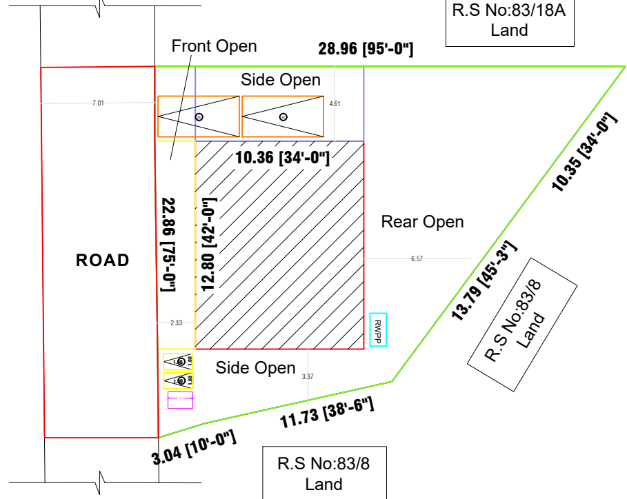
SITE PLAN
