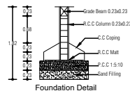
Foundation Detail
