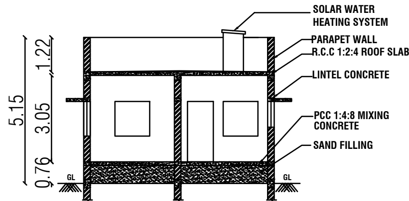
SECTION NO -"AB"
