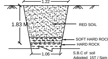
TRIAL PIT DETAILS NOT TO SCALE
