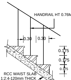
STAIR CASE STEPS SCALE 1:25
