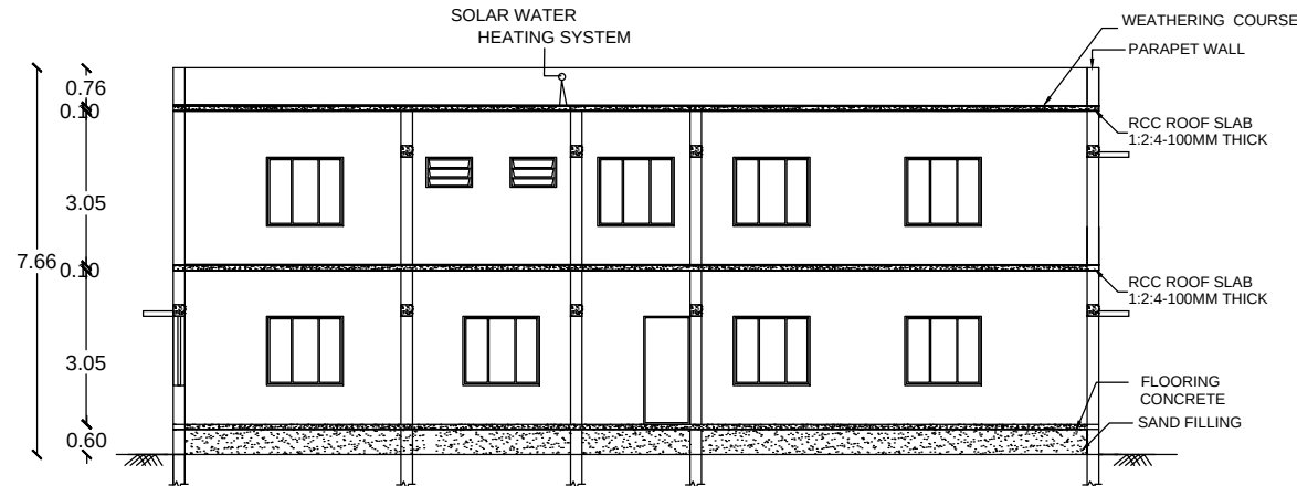
SECTION ON RM
