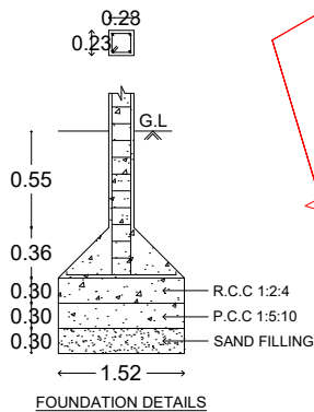
FOUNDATION DETAILS
