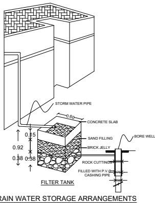
RAIN WATER STORAGE ARRANGEMENTS
