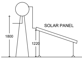
SIDE ELEVATION [ Not to scale ]
