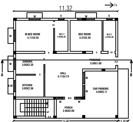
EXI.GROUND FLOOR PLAN
