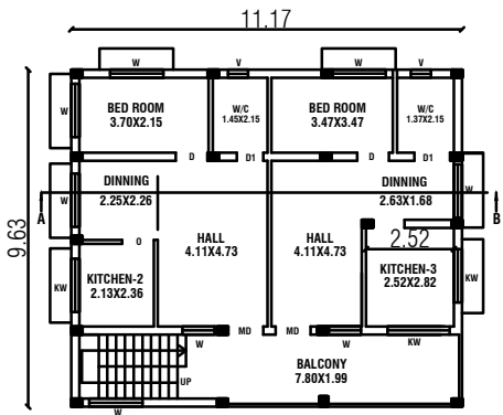
PRO.SECOND FIRST FLOOR PLAN
