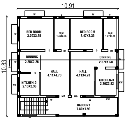
EXI.FIRST FLOOR PLAN
