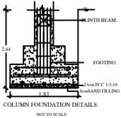
COLUMN FOUNDATION DETAILS NOT TO SCALE
