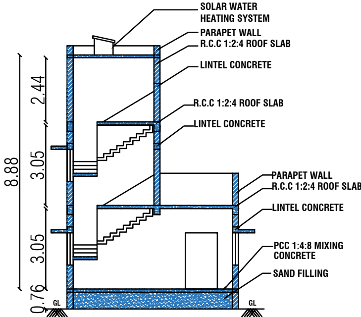
SECTION NO -"AB"
