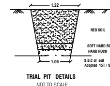
TRIAL PIT DETAILS NOT TO SCALE
