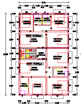
PRO. SECOND FLOOR
