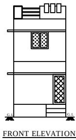
FRONT ELEVATION
