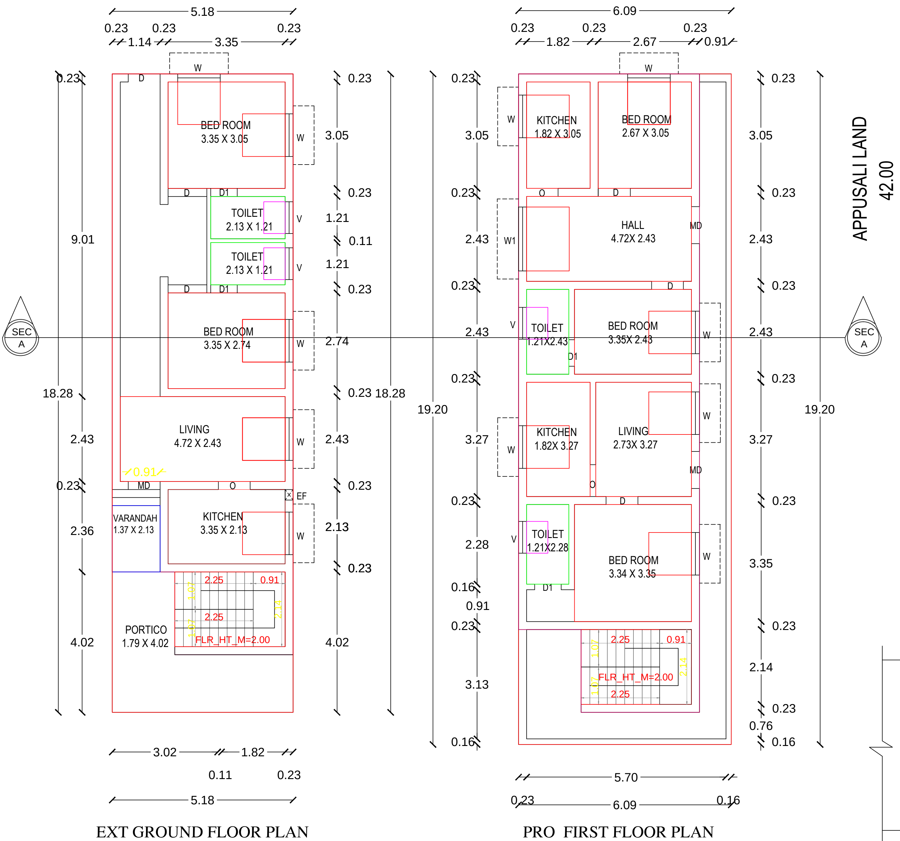
EXT GROUND FLOOR PLAN
