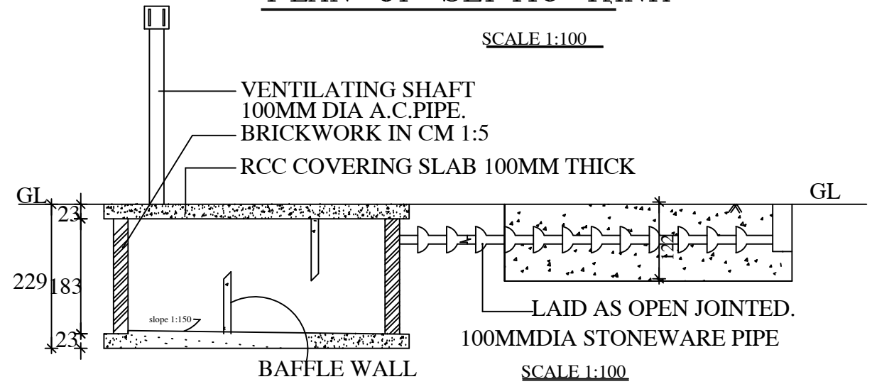
SECTION OF SEPTIC TANK (Not to scale)
