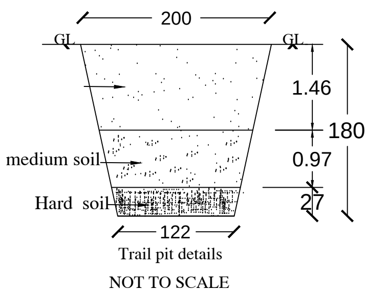
Trail pit details NOT TO SCALE
