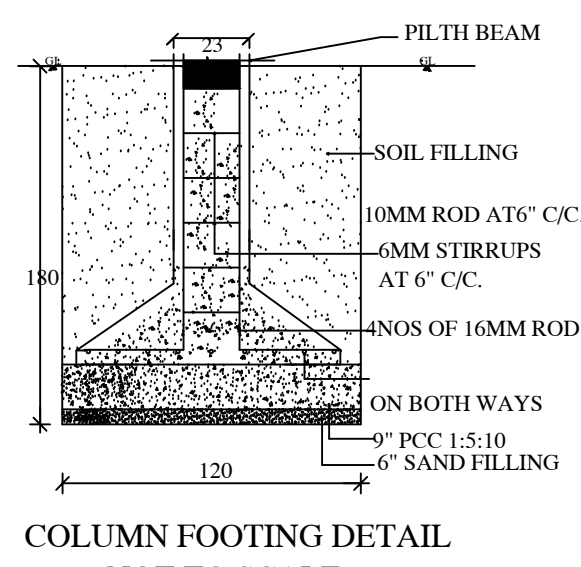
COLUMN FOOTING DETAIL NOT TO SCALE
