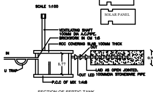
SECTION OF SEPTIC TANK
