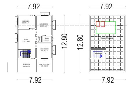
PRO.GROUND FLOOR PLAN OPEN TERRACE
