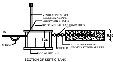
SECTION OF SEPTIC TANK
