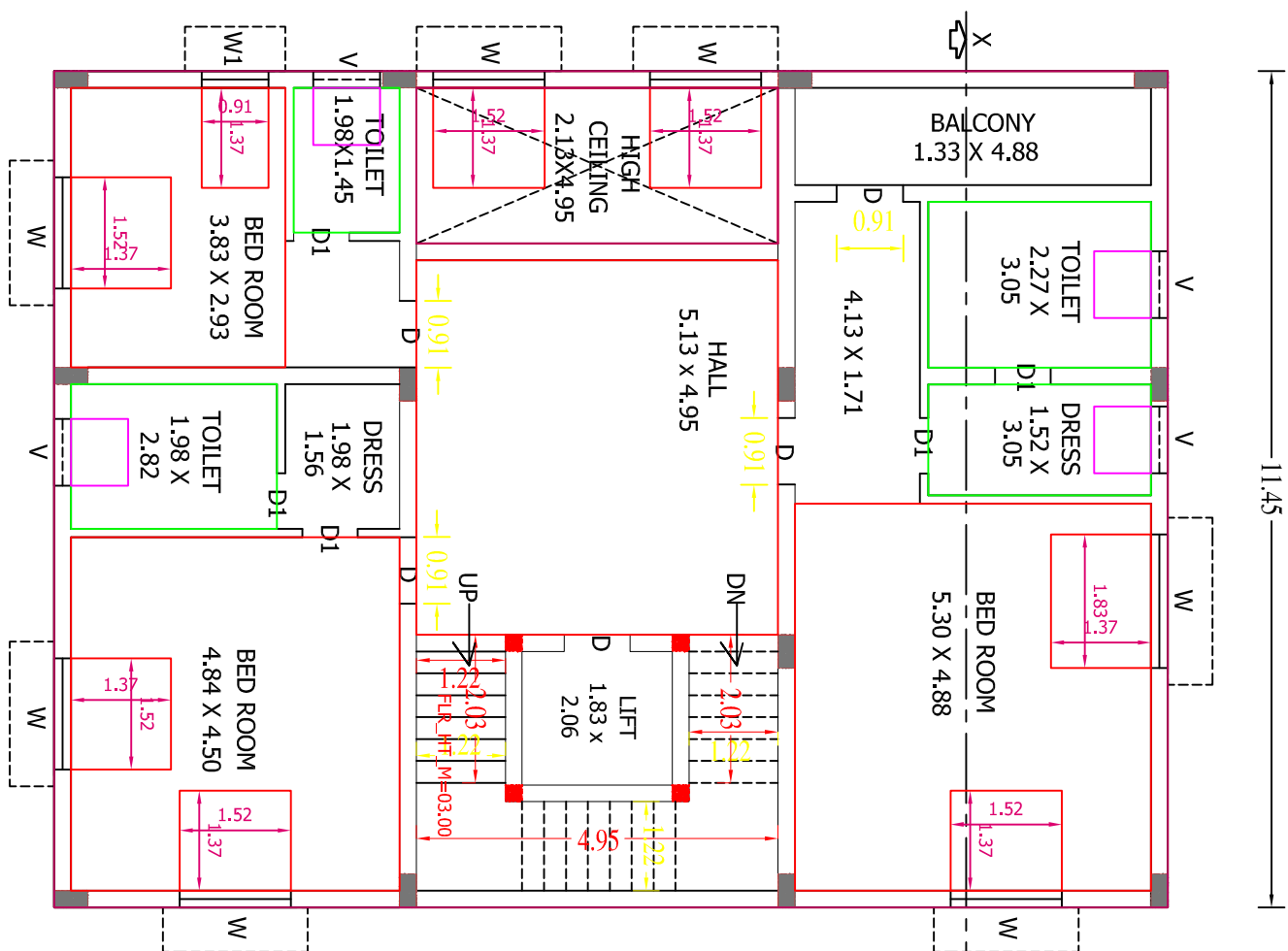
PRO. SECOND FLOOR PLAN
