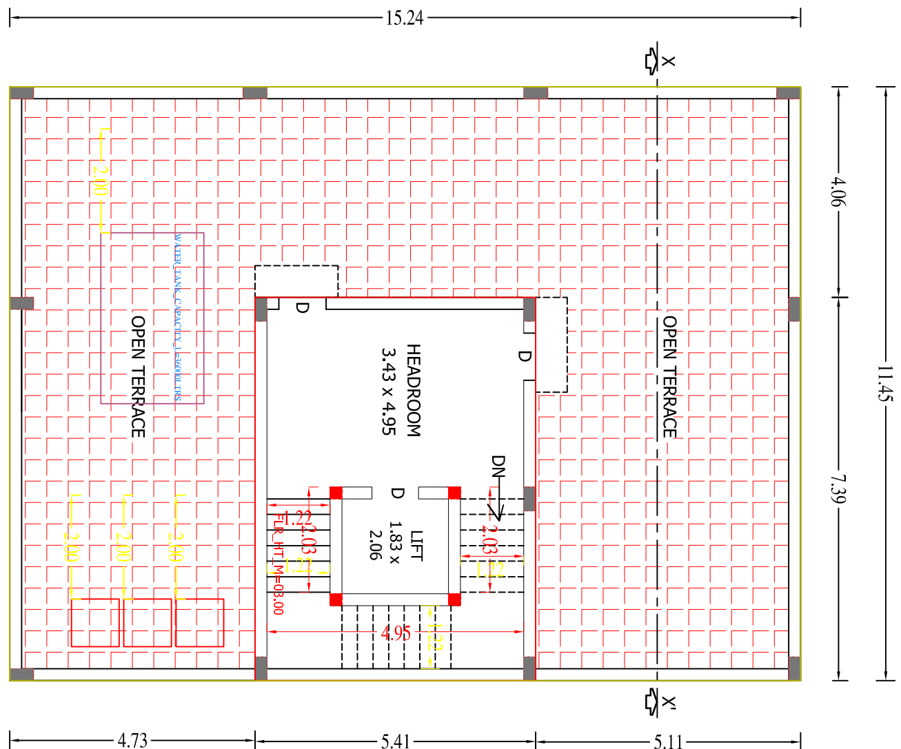
PRO. TERRACE FLOOR PLAN
